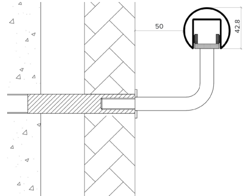
Wall Bracket
